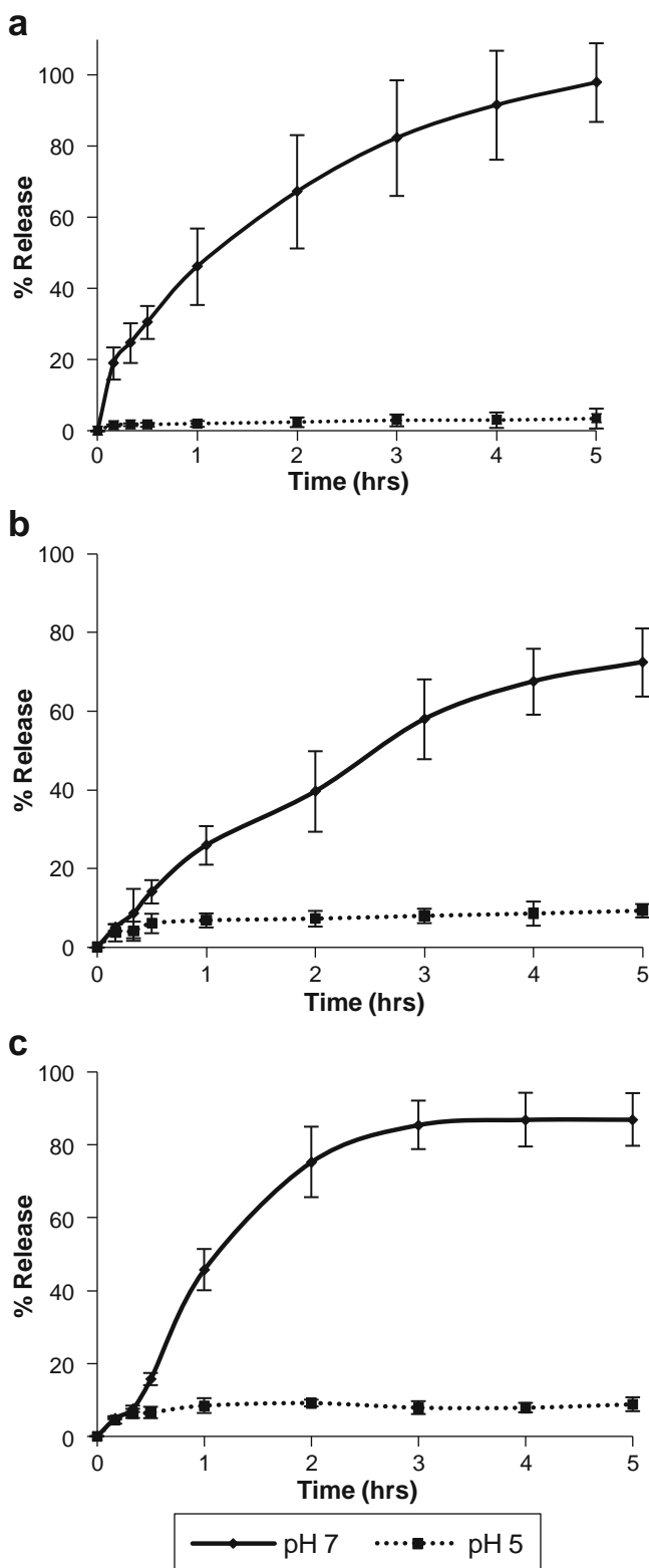
Fig. 2 Release of hydrocortisone from (a) Carbopol hydrogel, (b) neutralised Carbopol hydrogel and (c) HPMC gel. Results are presented as mean \pm SD, n=3-5 .
